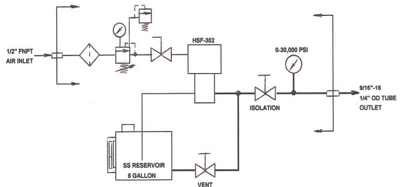
PORTABLE TEST CART FOR WATER SERVICE UP TO 25,000 PSI
